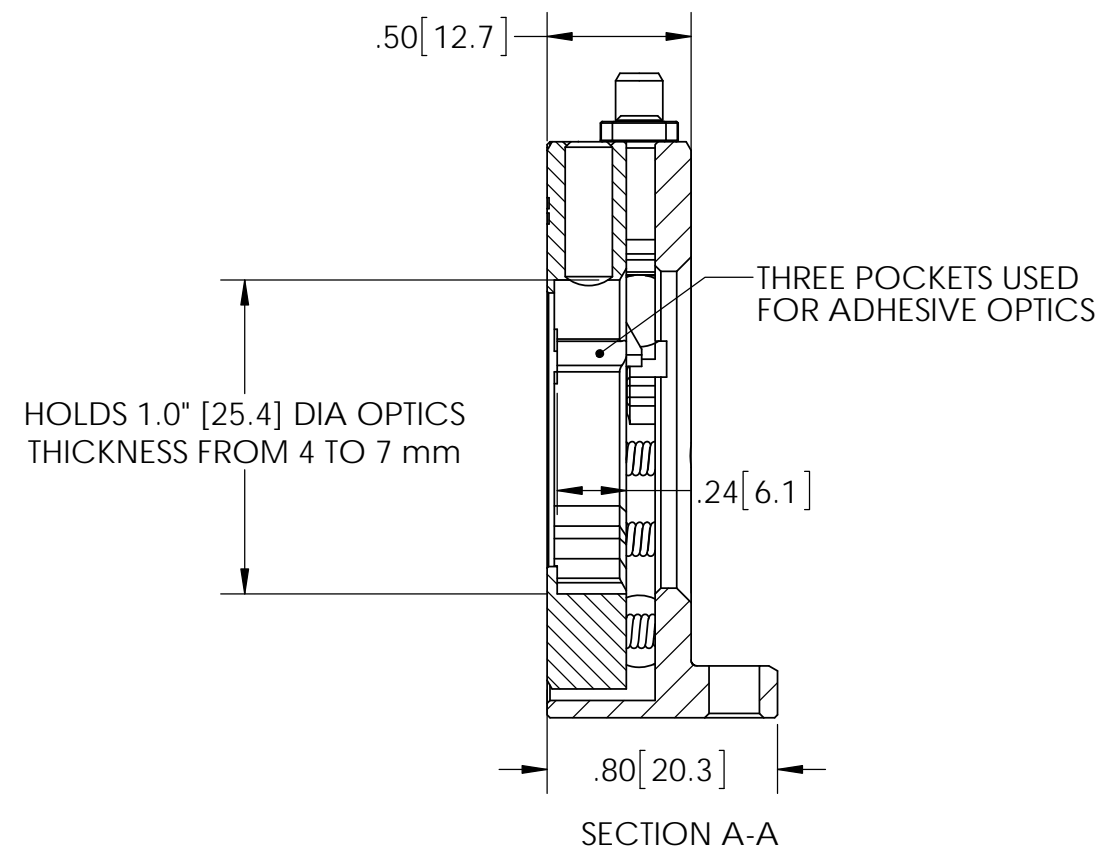
MODEL: HVM-S1r REAR LOAD
