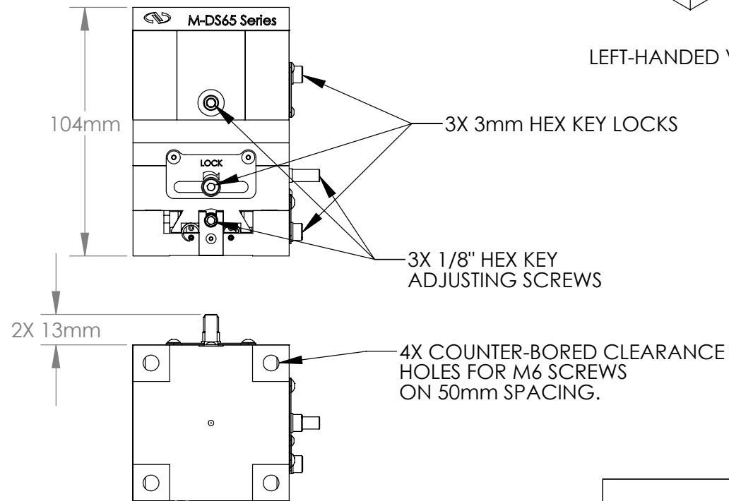
BOTTOM VIEW
