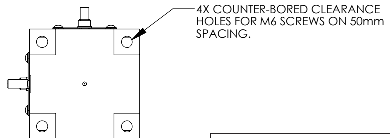
BOTTOM VIEW
