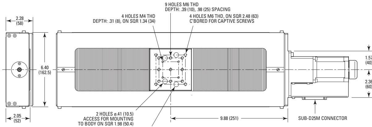
MODEL SHOWN: MTN300PP DIMENSIONS IN INCHES (AND MILLIMETERS)
