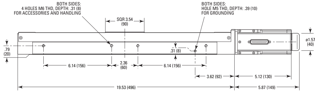
MODEL SHOWN: MTN300PP DIMENSIONS IN INCHES (AND MILLIMETERS)
