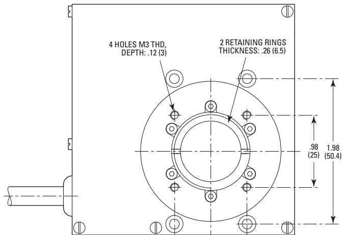
TOP VIEW SHOWN WITH RETAINING RINGS
