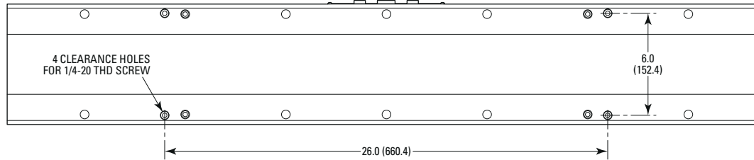
VIEW A
