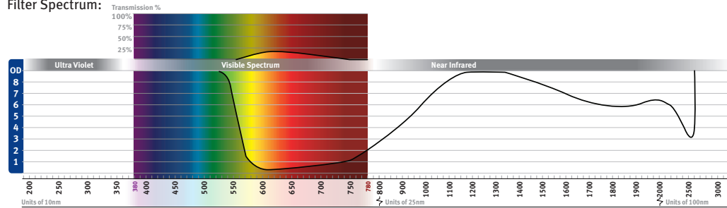
Filter Spectrum:
