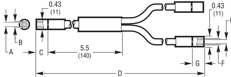
77533 BIFURCATED GLASS BUNDL E
