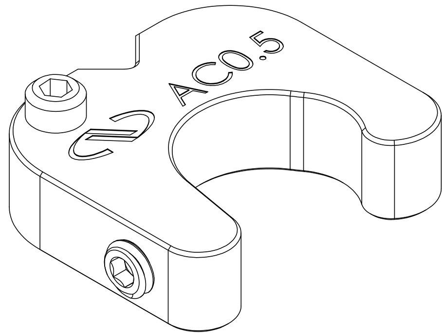
MODEL AC0.5
