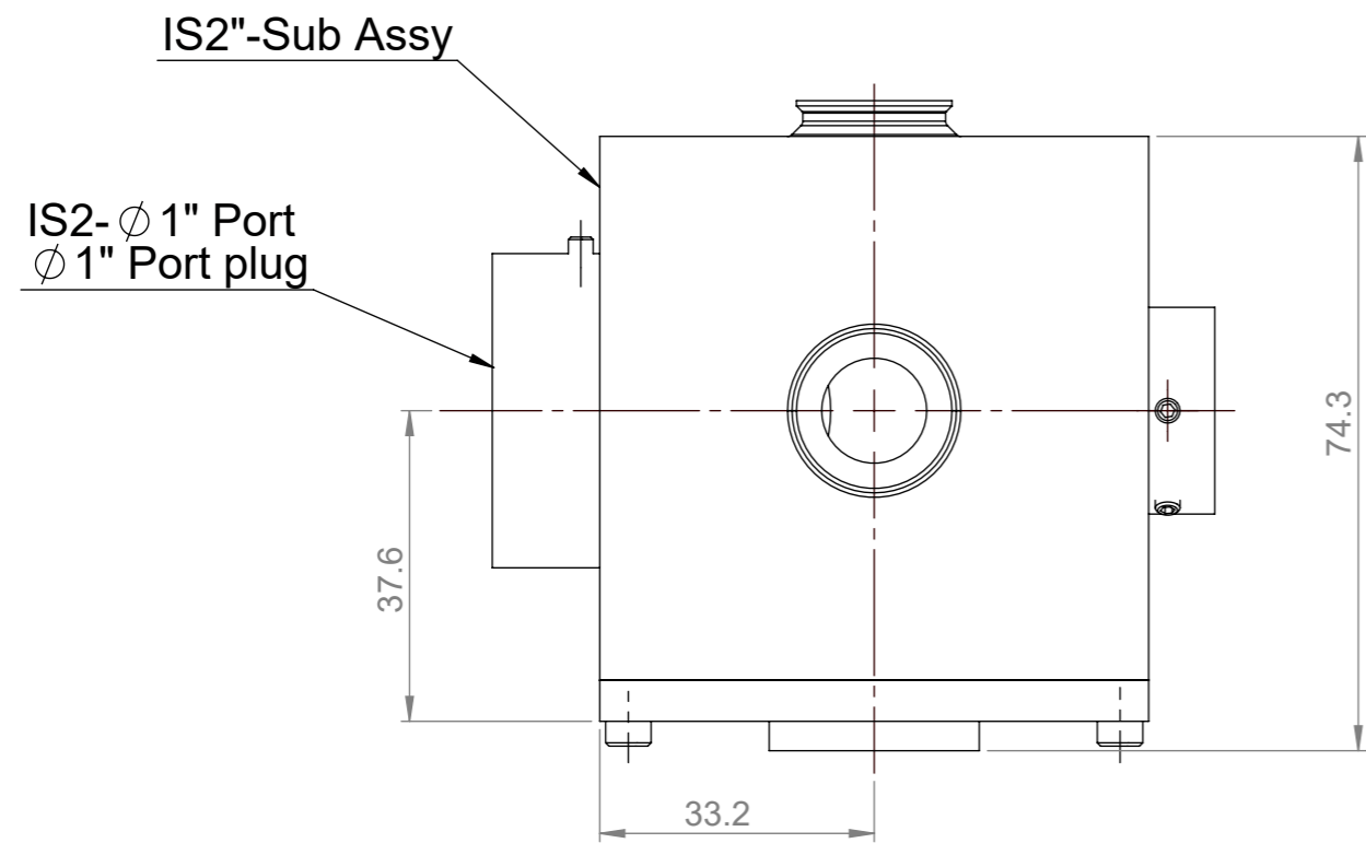
Front View
